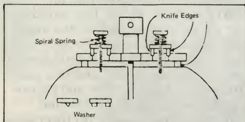
Fig. 1. An improved form of helical-spring pivot introduced by Perophone in 1927. A washer with its own pair of fulcra is inserted between the spring and the stylus-mount or pressure-plate.
